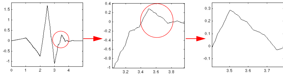
Figure 6-9: Zooming in on a db3 Wavelet
