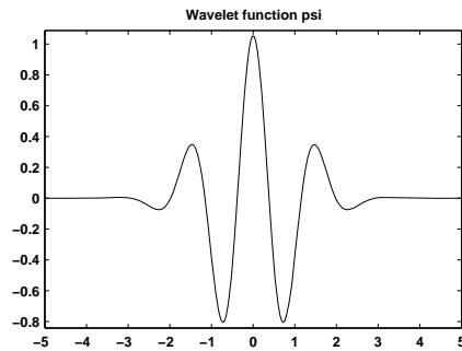
Figure 6-20: Gaussian Derivative Wavelet gauss
