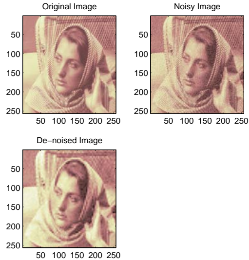
Figure 6-31: Image De-Noising
